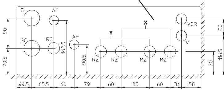
REAR CONNECTION
