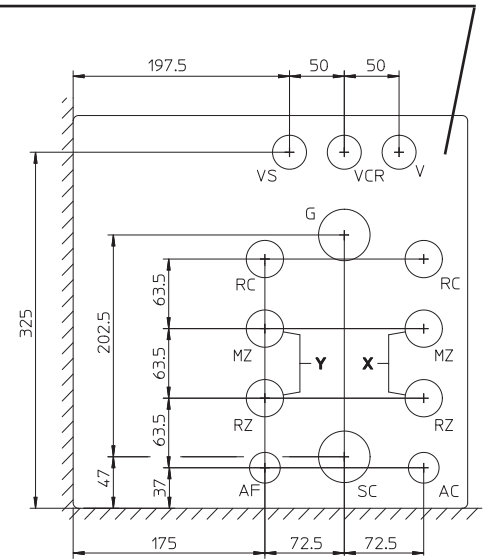
RIGHT HAND SIDE CONNECTION
