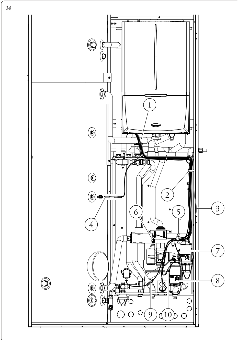
DHW probe - positioning (Det. 4)
