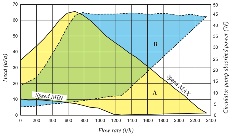
Proportional head ( \Delta P V ).
