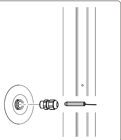
DHW probe - positioning (Det. 4)
