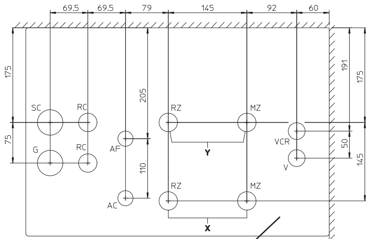
LOWER CONNECTION
